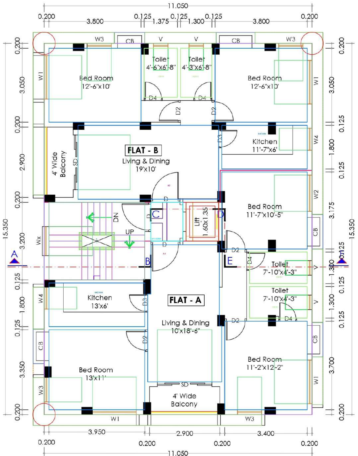
TYPICAL 1ST TO 3RD FLOOR PLAN
